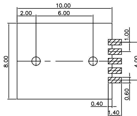
PCB LAYOUT TOLERANCE:±0.1 LAND METAL MASK t=0.12
