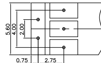
FILM CONTACT LAYOUT TOLERANCE:±0.1
